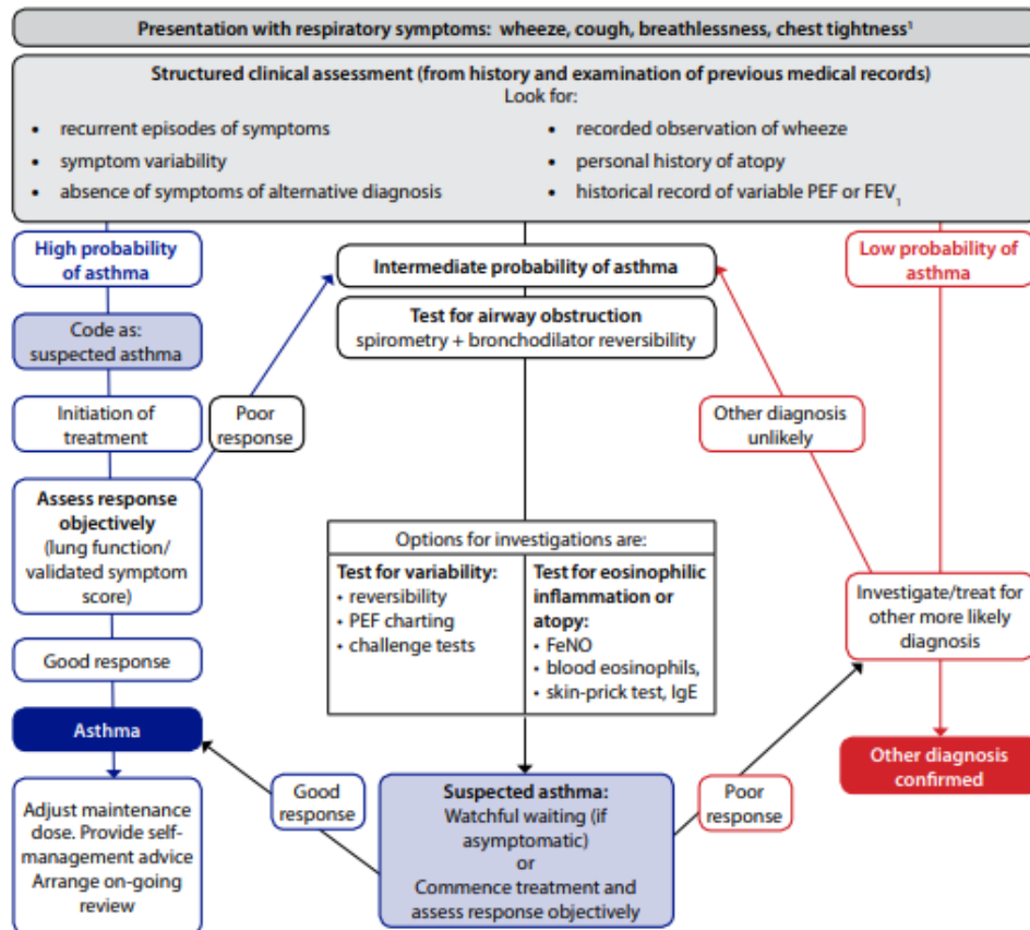
Figure 1: Diagnostic algorithm
