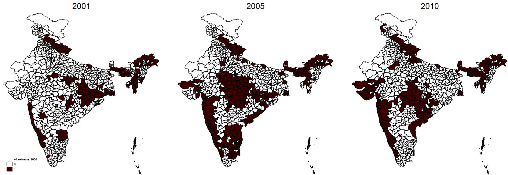
Figure 2: Maps of Extreme Precipitation Events
