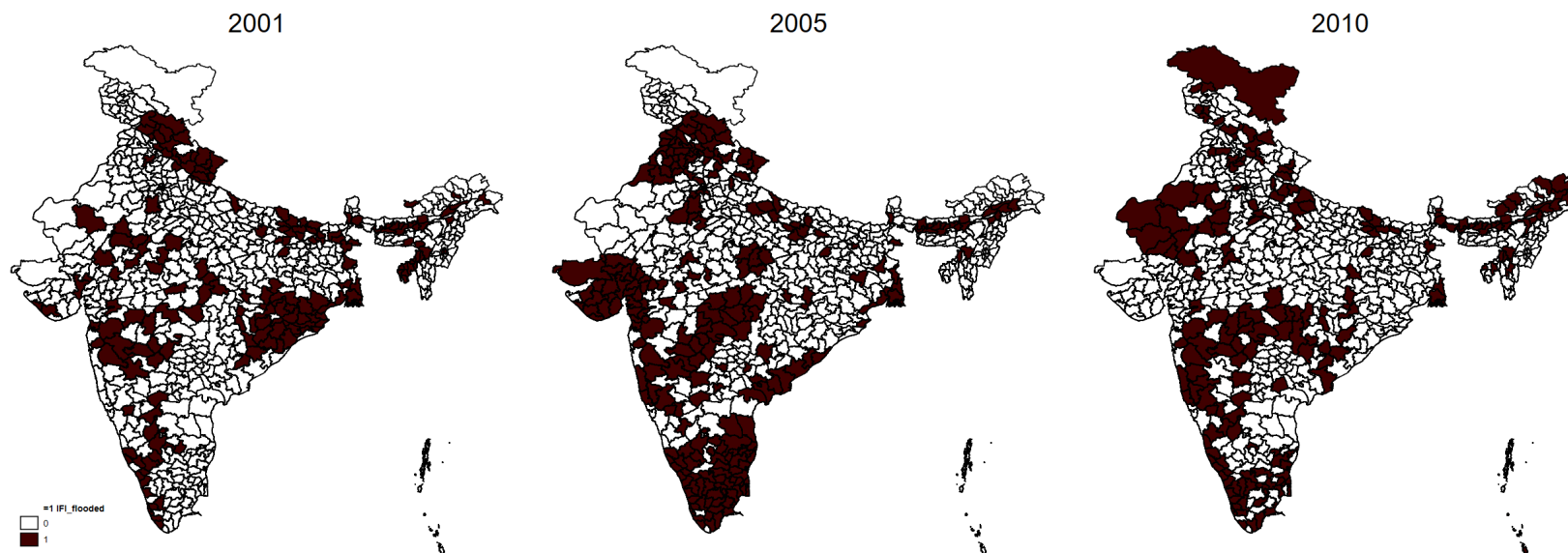
Figure 7: Maps of Flood Events
